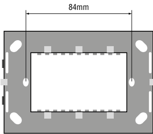
Assembly dimensions
