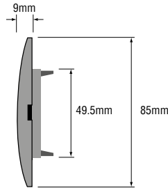
Surround dimensions
