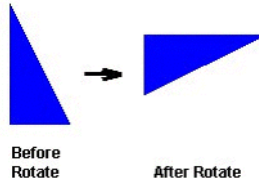
Rotating Objects
