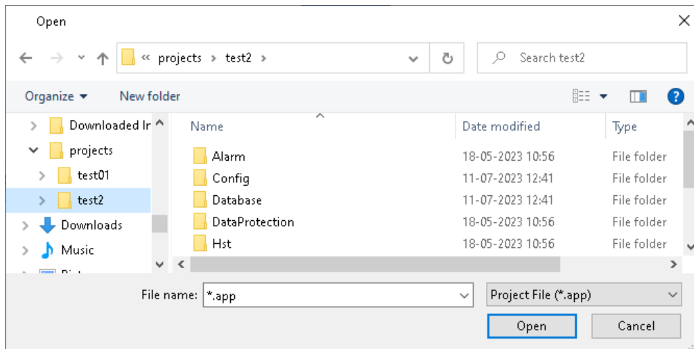
Open dialog
