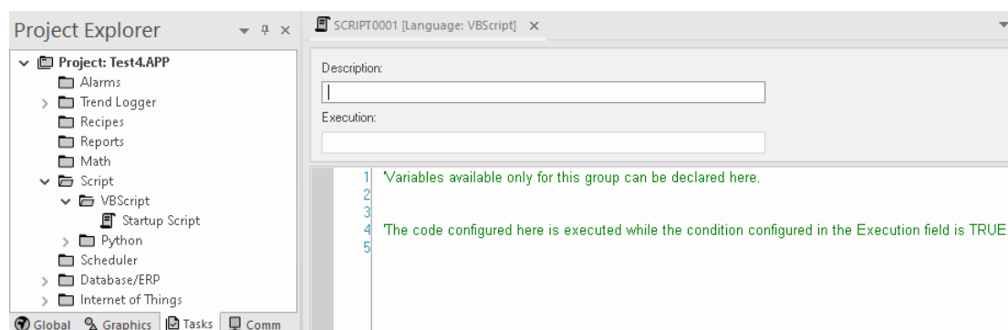
Script worksheet
