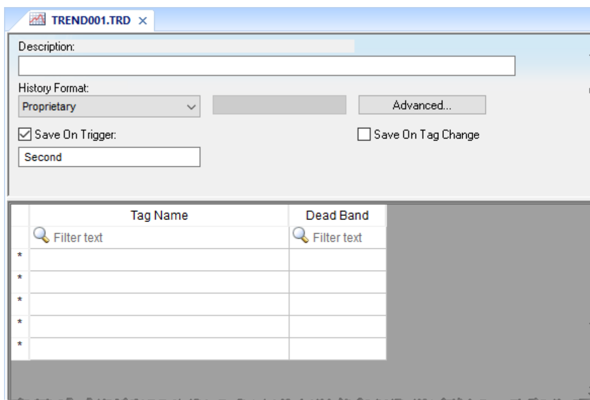
Trend worksheet
