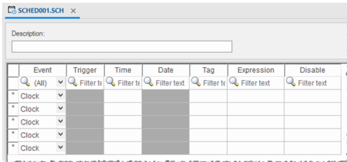
Scheduler worksheet
