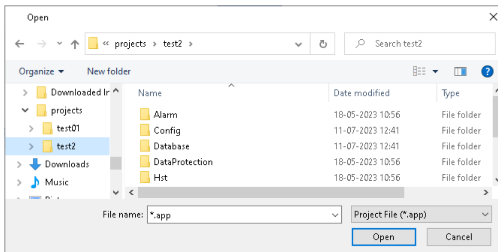
Open dialog
