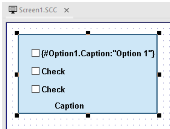
Updated Symbol
