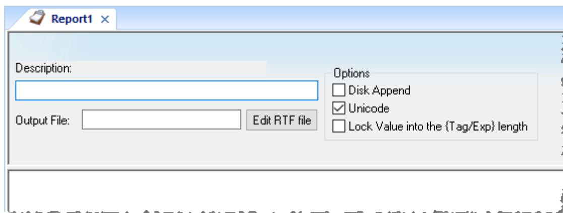
Report worksheet
