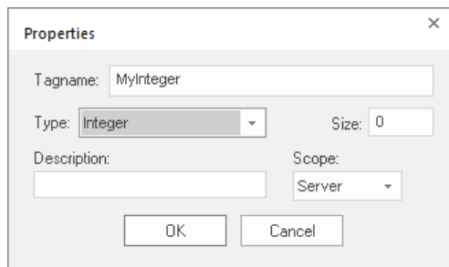
Properties dialog
